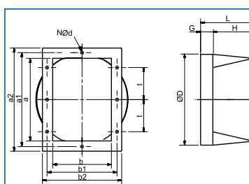
ACP-N Outlet transformation connector. Provided with a sliding blade to control the air volume.
