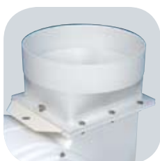
ACP-N Outlet transformation connector. Provided with a sliding blade to control the air volume.
