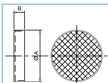
DEF-CIR Protection guard To prevent any contact with the impeller fan. To install at the inlet side.
